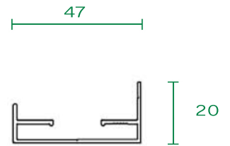
Side Frames
