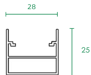
Bottom Track
