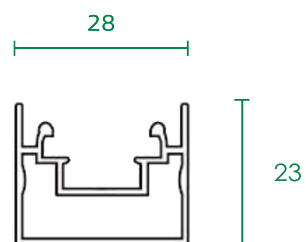
Side Frames
