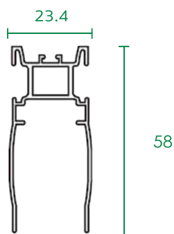
Handle
